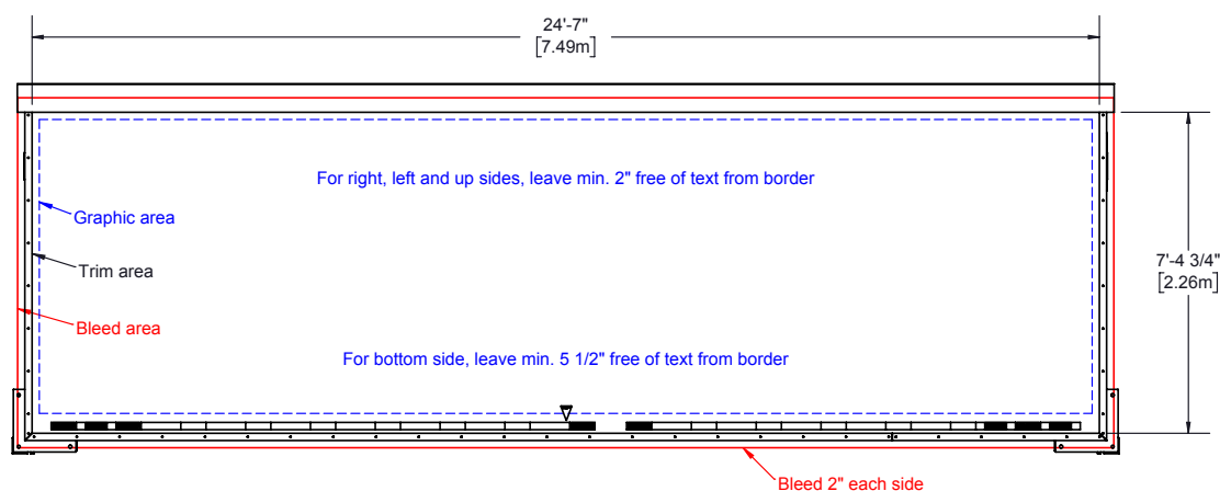
SIDE PANEL SCALE 1:50 QTY. 2
