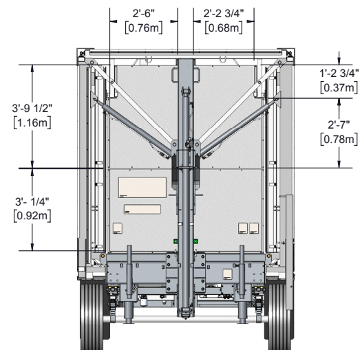
FRONT VIEW SCALE 1:50
