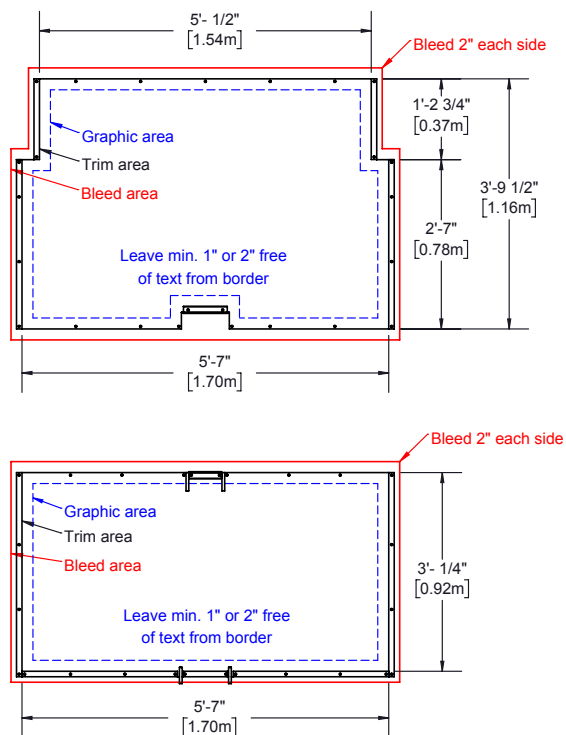
FRONT VIEW REAR VIEW SCALE 1:30
