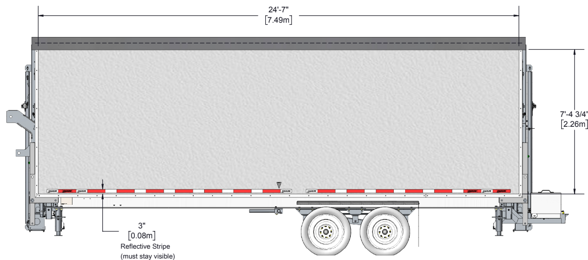
SIDE VIEW SCALE 1:50
