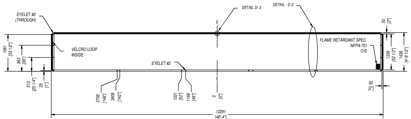
SKIRT (outside view)
