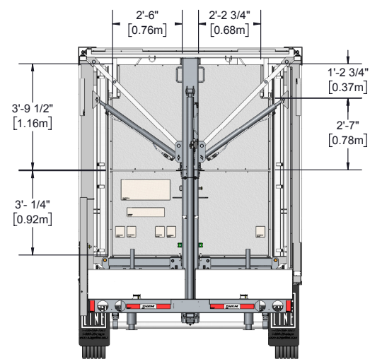
REAR VIEW SCALE 1:50
